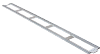
TRO-0475-13-00-00-0 Schienenmontage 1800mm (70,9") V" Nutmittellinie 152 mm (6")
