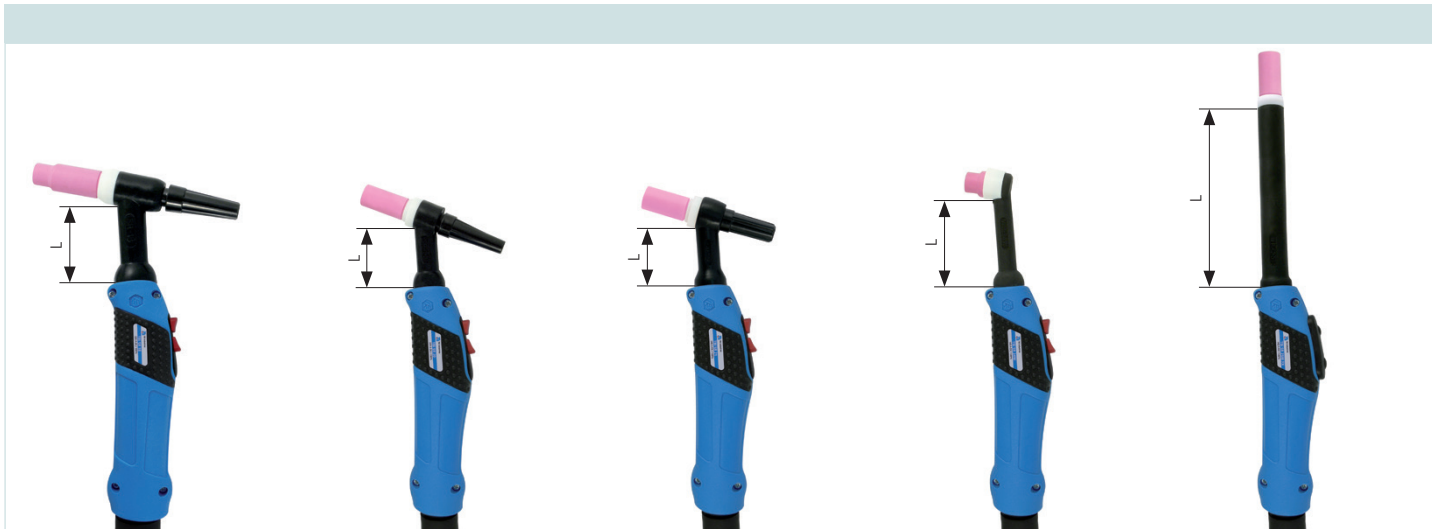
TBi SR 18 (FX) TBi SR 18 V (FX) 100% (10 min.) AC: 225 A DC: 320 A Ø 0.5-4.0 mm L = 50 mm (FX: 50 mm)
