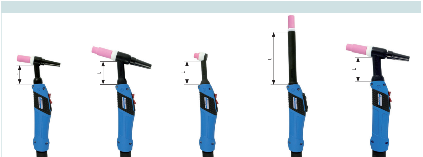
TBi SR 9 (FX) TBi SR 9 V (FX) 60% (10 min.) AC: 80 A DC: 110 A Ø 0.5-1.6 mm L = 35 mm (FX: 35 mm (Std.), 115 mm)
